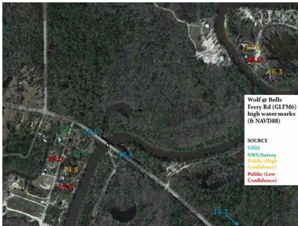
Figure 9. High water marks near the Wolf River at Bells Ferry Rd (GLFM6) gauge color-coded by confidence level. High water marks were adjusted to NAVD88 based upon the assumed staff gauge datum of -1.0 ft NAVD88.
