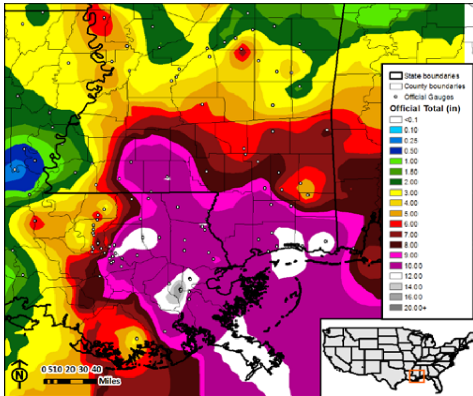
Figure 13. Storm total rainfall as observed by official precipitation gauges. Observations were interpolated by the Kriging method.
