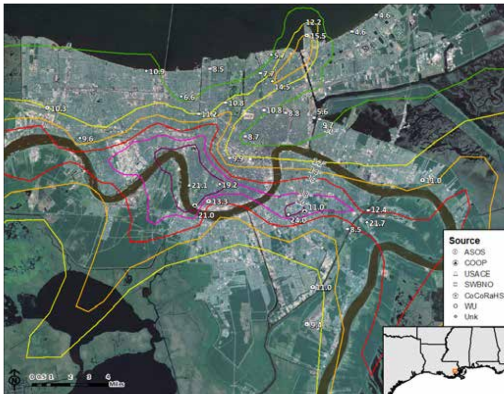
Figure 16. Storm total rainfall reported from all official and private gauges in the New Orleans area during Hurricane Isaac. Contours were produced from a Kriging interpolation of all official and private gauges. Note the particularly high values evident along the Mississippi River from roughly Gretna to Audubon Park.
