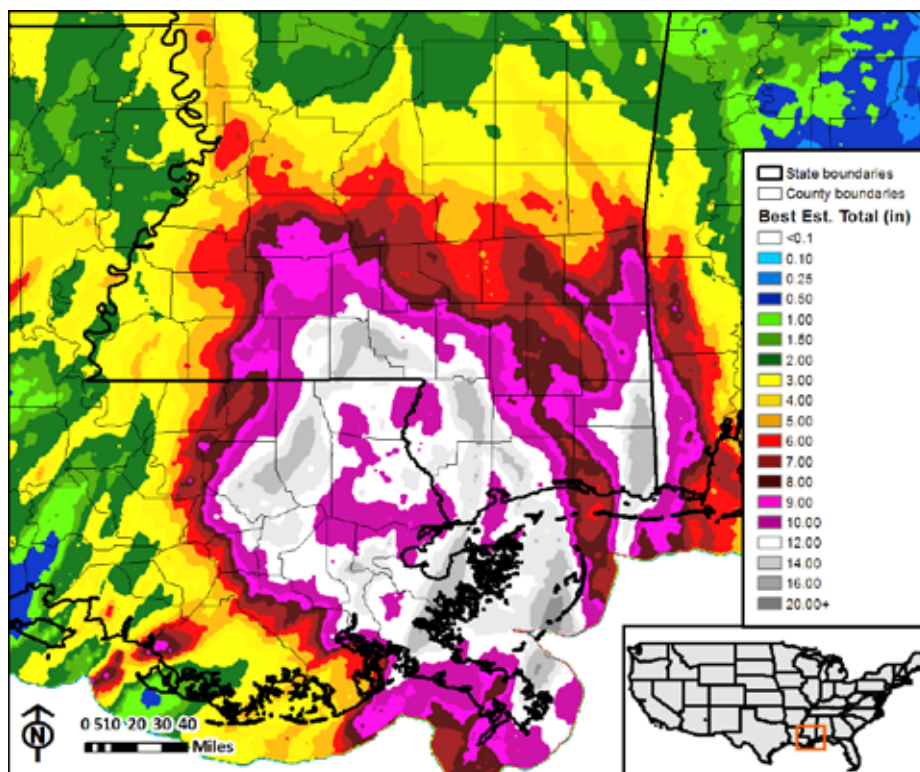
Figure 14. Storm total rainfall as estimated by a combination of official gauges, radar data, and forecaster experience in the NWS RFC QPE product.
