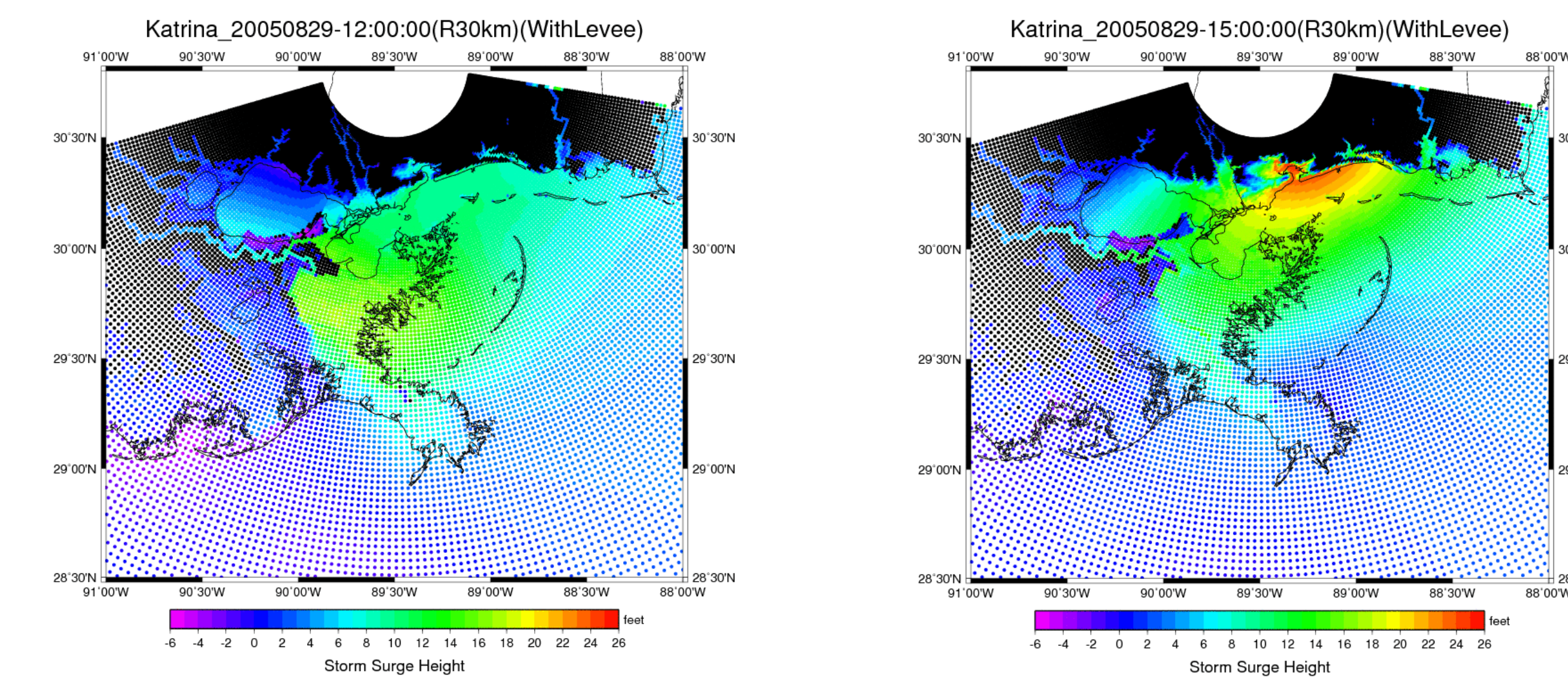
Figure 2. Katrina's storm surge in control run at 12 UTC and 15 UTC 29 August 2005 (ft).
