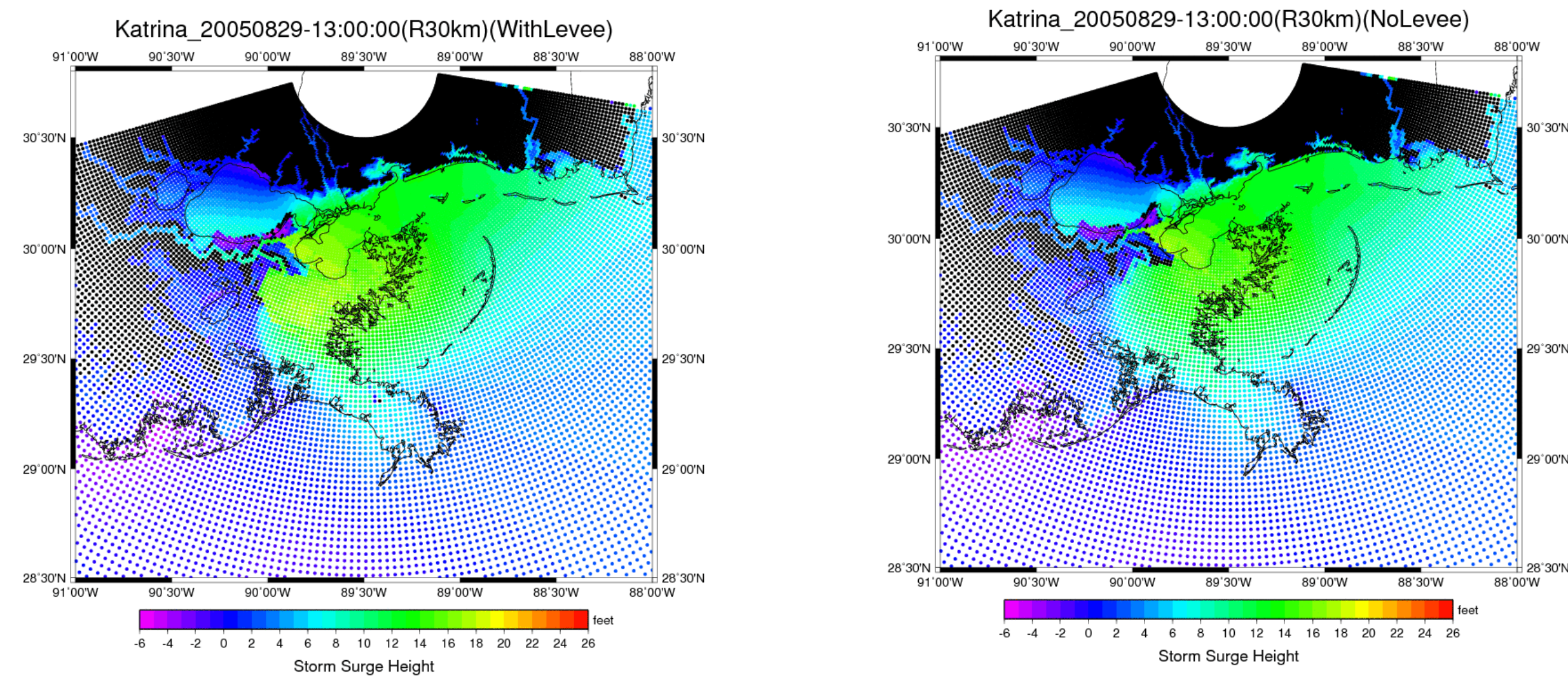
Figure 3. Katrina's storm surge in control run at 13 UTC compared to same simulation without a man-made levee along the Mississippi River up to Chalmette.
