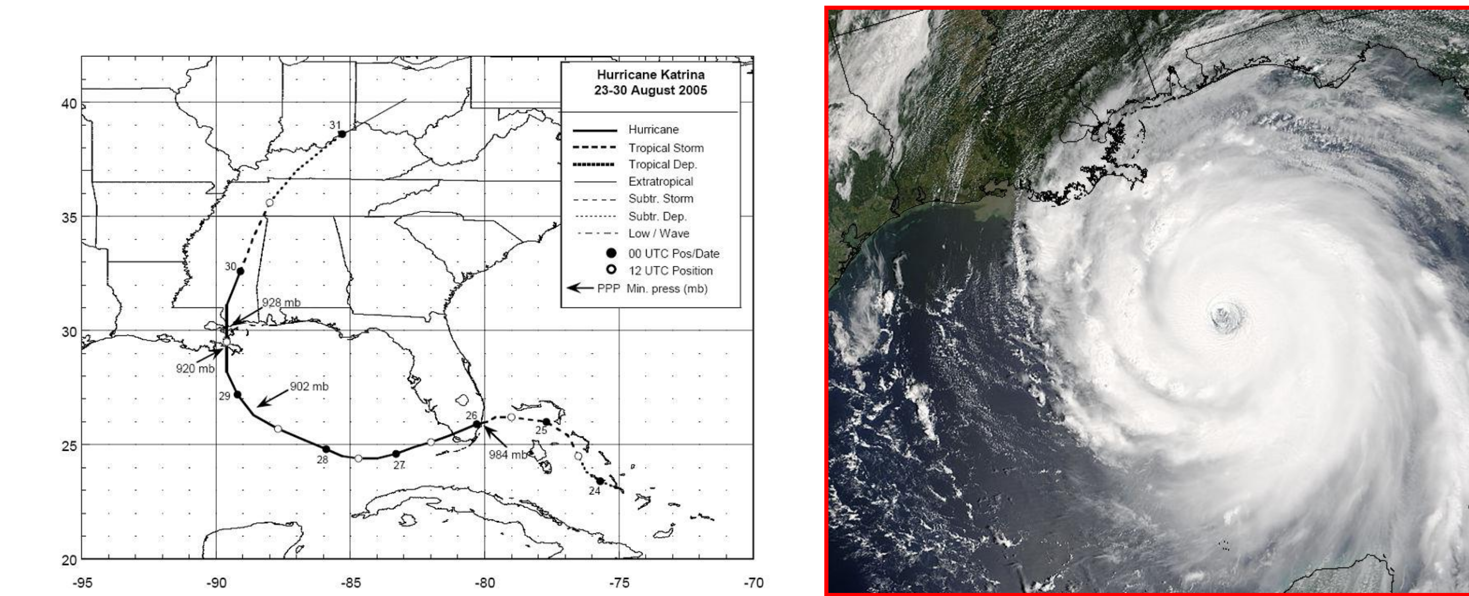
Figure 1. Best track position map prepared by the National Hurricane Center (left) and MODIS-Terra image of Hurricane Katrina (right).
