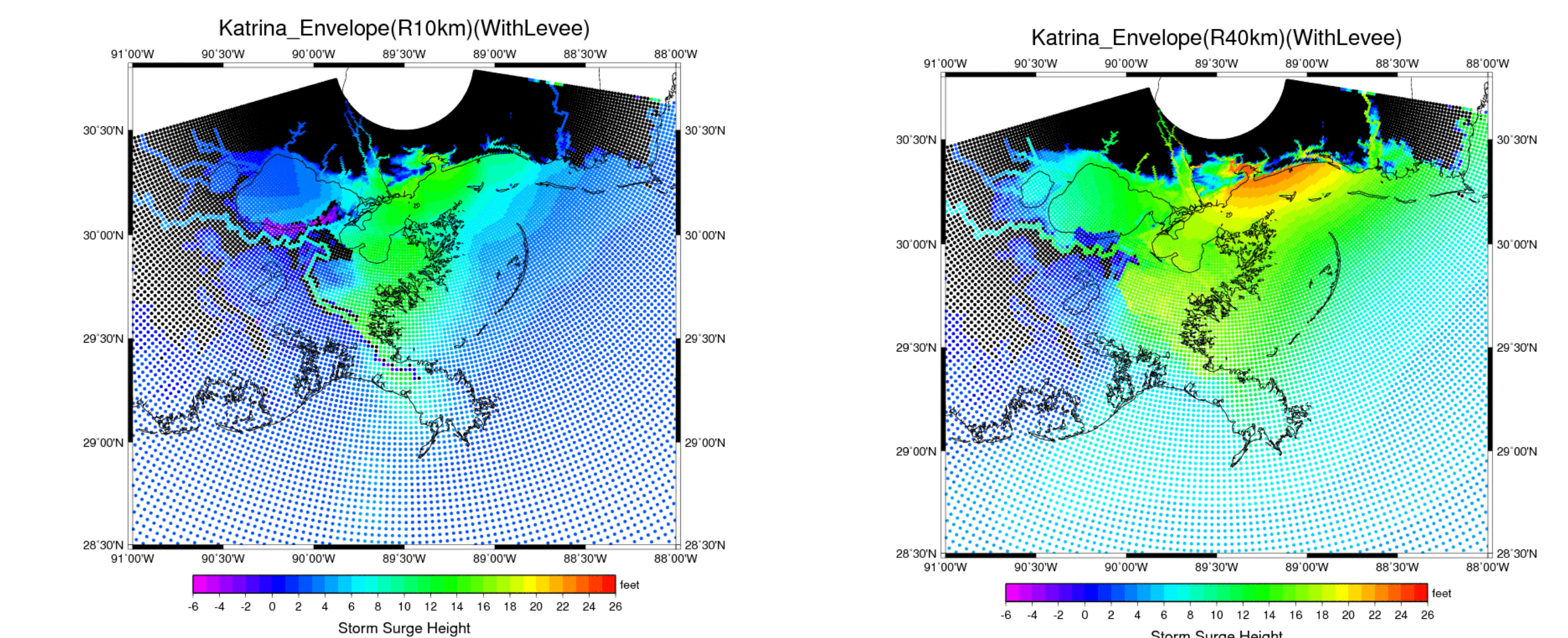
Figure 6. Peak storm surge values for a small (left) and large (right) hurricane with a pressure deficit similar to Katrina.
