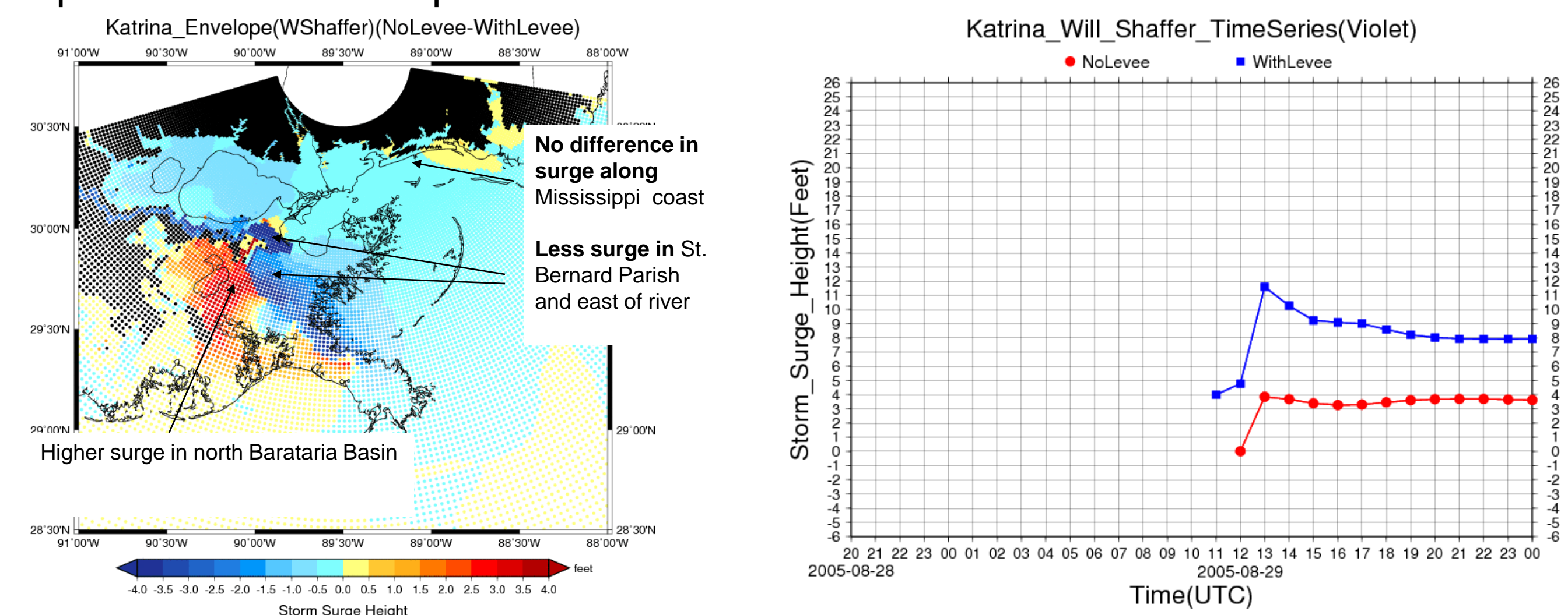
Figure 5. Times series of storm surge near Violet, LA, in St. Bernard Parish with and without the Mississippi River levees as water flowed over the Chalmette levee system.
